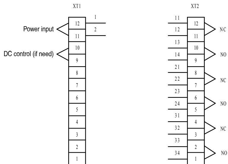
EVC5 series electric holding type vacuum contact or wiring terminal scheme
