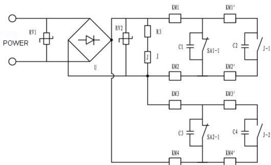
GVC611 series vacuum contactor schematic diagram
