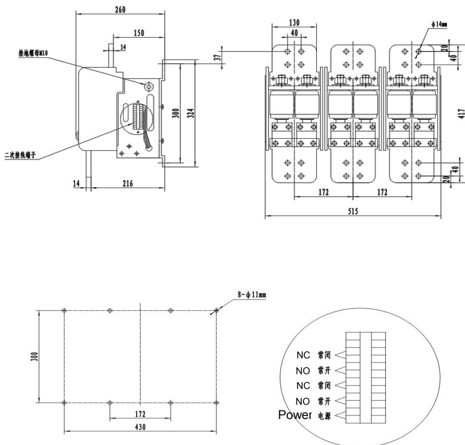
GVC611 series vacuum contactor outline drawing
