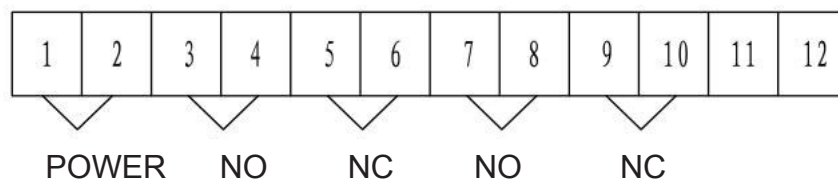
GVC611 series vacuum contactor wiring diagram
