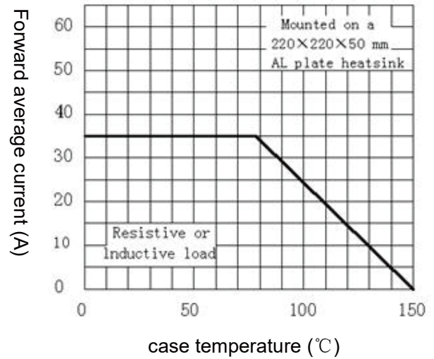
Case temperature vs forward average current
