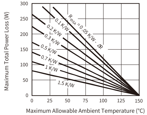
Fig. 3 - Total Power Loss Characteristics
