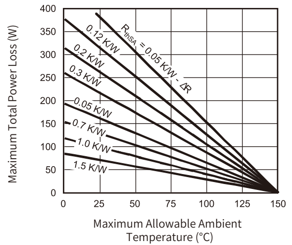
Fig. 3 - Total Power Loss Characteristics
