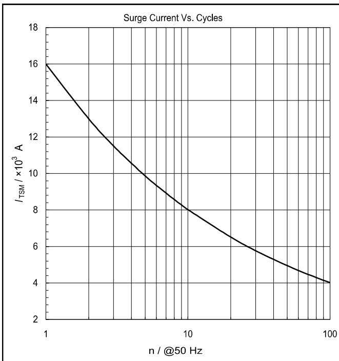
Fig5. Surge Current Vs. Cycles
