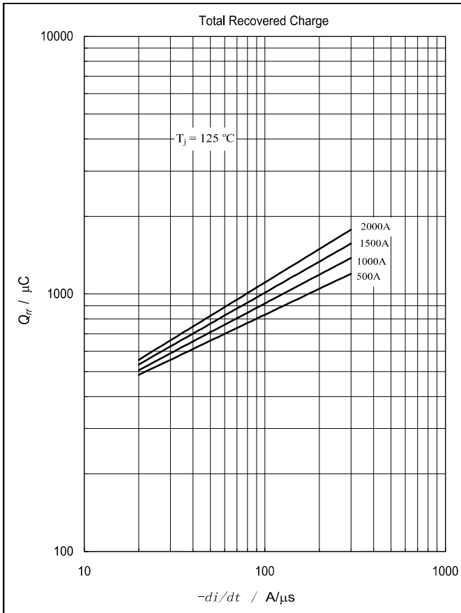
Fig3. Total Recovered Charge Vs. Commutation Rate
