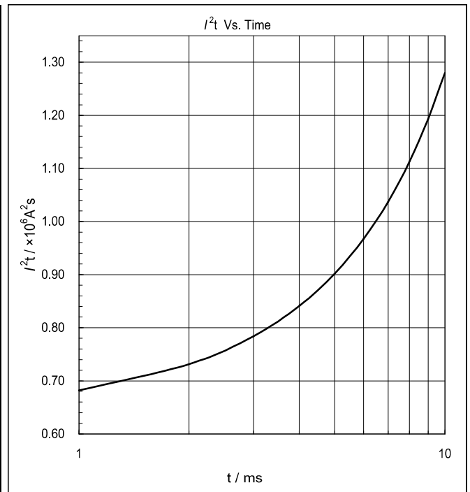
Fig6. I^2t Vs. Time
