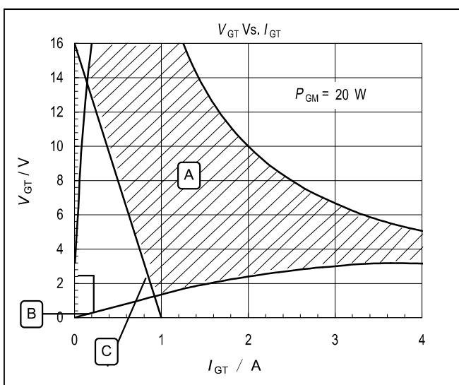
Fig8. V_{GT} Vs. I_{GT}
