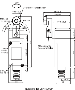
Nylon Roller LSN-5000P
