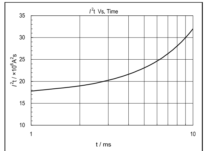
Fig4. I 2 t Vs. Time
