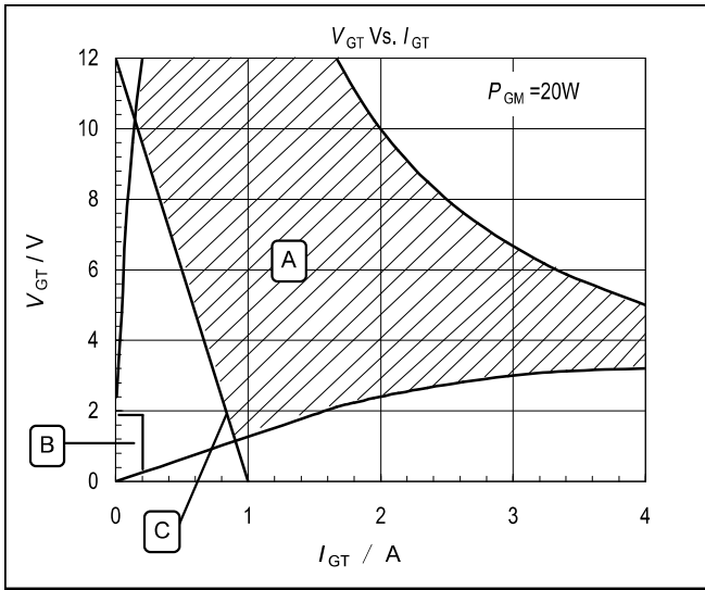
Fig9. V_{GT} Vs. I_{GT}
