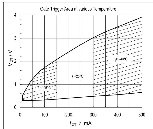
Fig12. Gate Trigger Area at various Temperature
