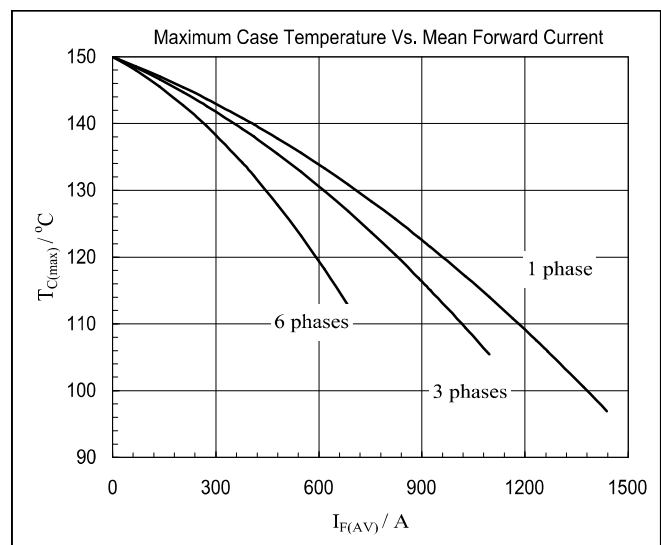
Fig4. Maximum Case Temperature Vs. Mean Forward Current
