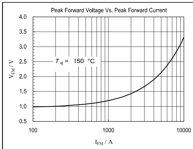
Fig1. Peak Forward Voltage Vs. Peak Forward Current
