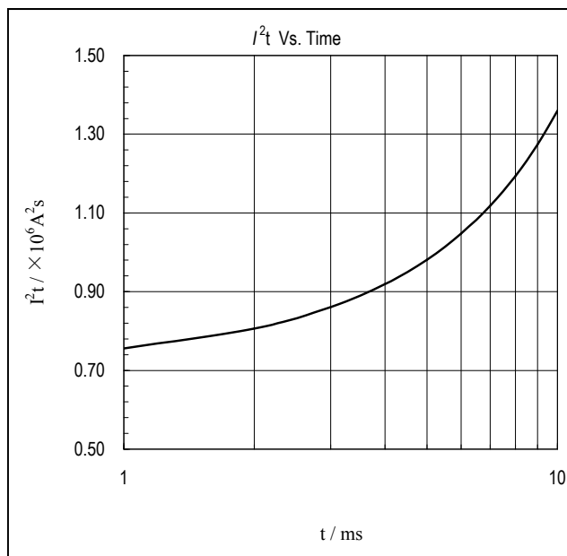
Fig6. I^2t Vs. Time
