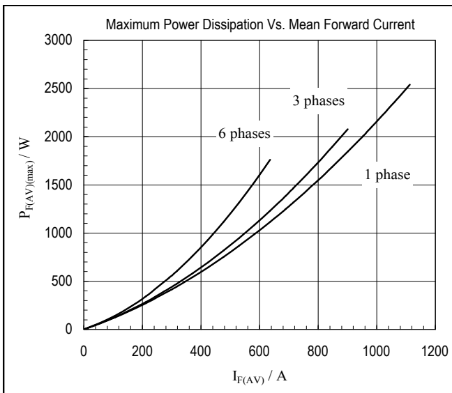
Fig3. Maximum Power Dissipation Vs. Mean Forward Current
