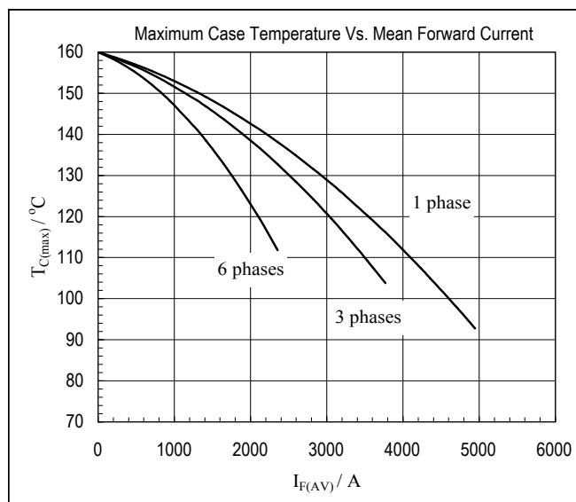
Fig4. Maximum Case Temperature Vs. Mean Forward Current
