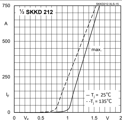
Fig. 15: Forward characteristics
