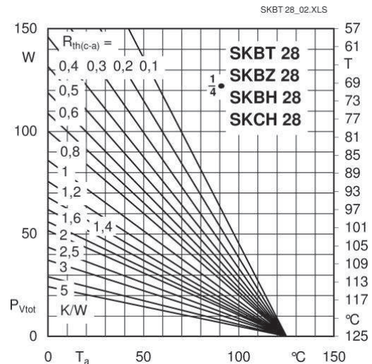
Fig. 2 Power dissipation vs. case temperature
