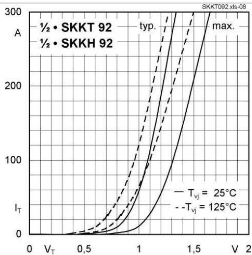
Fig. 7 On-state characteristics
